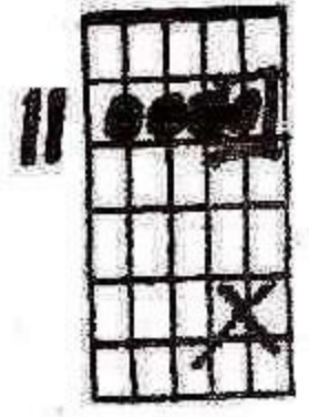
D#7sus 4
