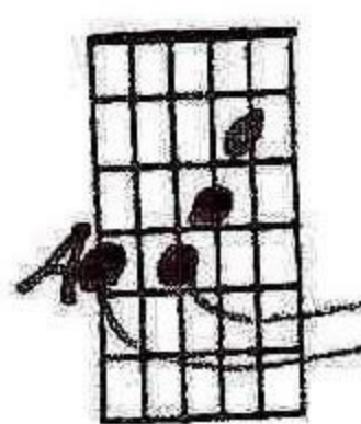
G#7sus 4
